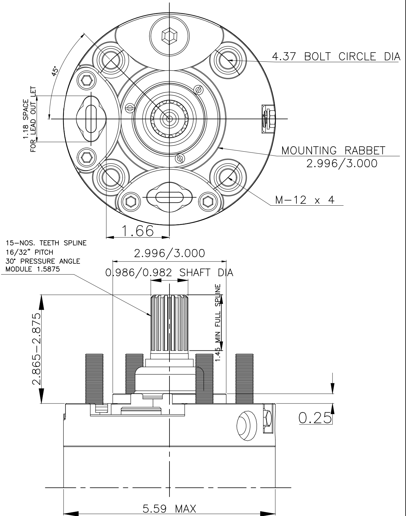
6" SUBMERSIBLE MOTOR ALL DIMENSIONS ARE IN INCH
